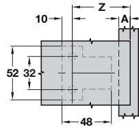
Screwing position
