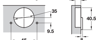
Drilling template 45/9.5 For screw fixing
