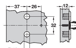
With dowel fixing
