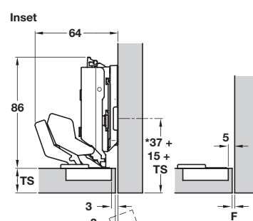
Mounting plate distance 6 mm *Dimension for mounting plate for 37 mm hole spacing
