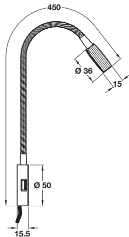
Loox5 12V LED 2034 flexible reading light with USB
