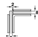
Glass machining without miter, 8 mm glass
