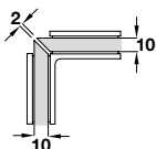
Glass machining with 45° miter, 10 mm glass
