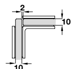
Glass machining without miter, 10 mm glass
