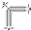
Glass machining with 45° miter, 8 mm glass
