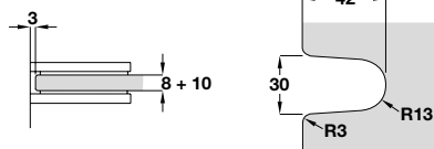
Glass machining
