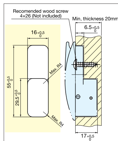
Bore Dimensions (For thickness 20~29mm)
