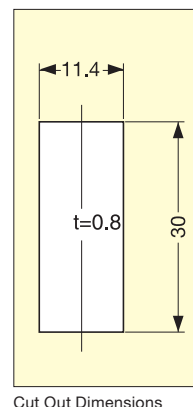
Cut Out Dimensions
