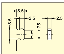
Recommended Strike Dimension
