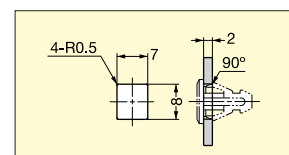
Cut Out Dimensions (Strike for metal)
