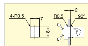
Cut Out Dimensions for body
