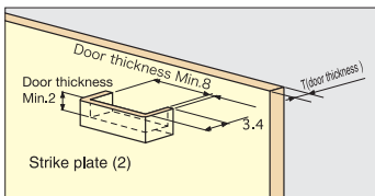
Recommended Strike Dimension
