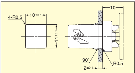
Cut Out Dimensions
