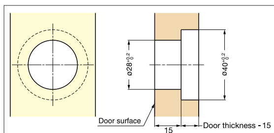
Bore Dimensions
