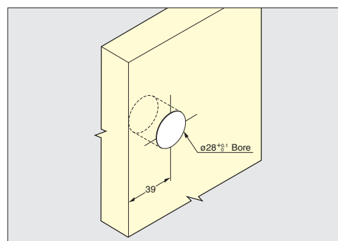
Bore Dimensions (Inset Door Application)
