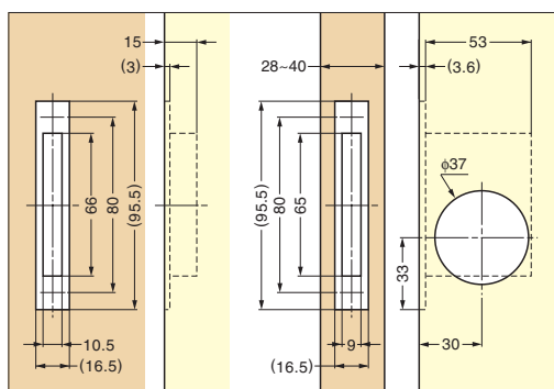
Bore Dimensions
