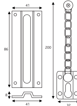
Slide Chain
