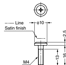
⑤ Truss head screw M4×16
