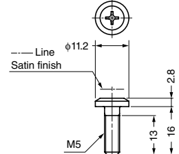
⑥ Truss head screw M5×16
