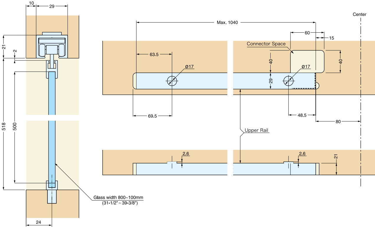
Dimensions (Left door)
