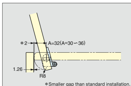
Installation with Rounded Lid Edge
