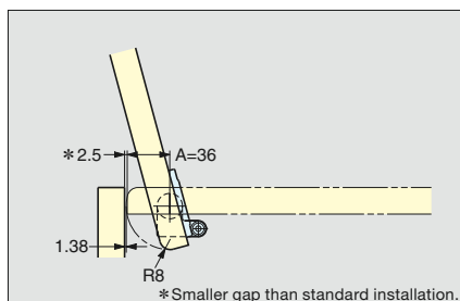
Installation with Rounded Lid Edge
