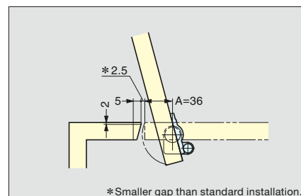
Installation with Inclined Edge
