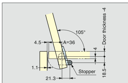
Standard Installation
